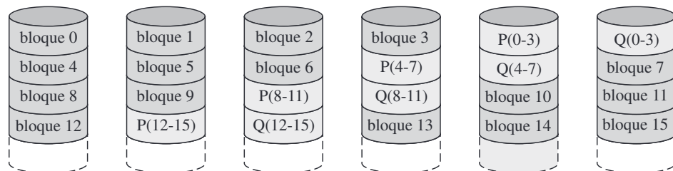
(g) RAID 6 (redundancia dual)
